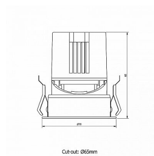
Cut-out: Ø65mm
