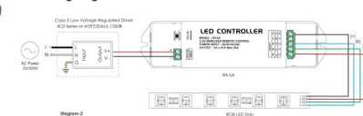
R4-5A Wiring Diagram
