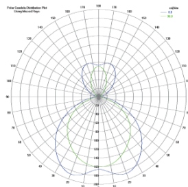
POWER LINE SLIM 30 DOUBLE
