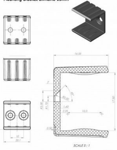
Mounting bracket SlimLine 15mm
